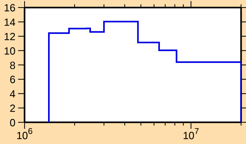
\Delta\sigma/\sigma vs. E for ^{184}\text{Pt}(n,\text{nonel.})
