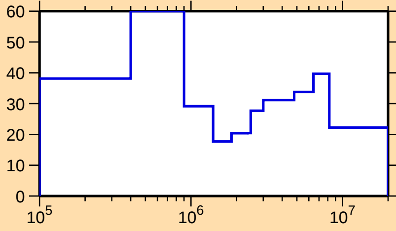
\Delta\sigma/\sigma vs. E for ^{184}\text{Pt}(n,\text{el.})
