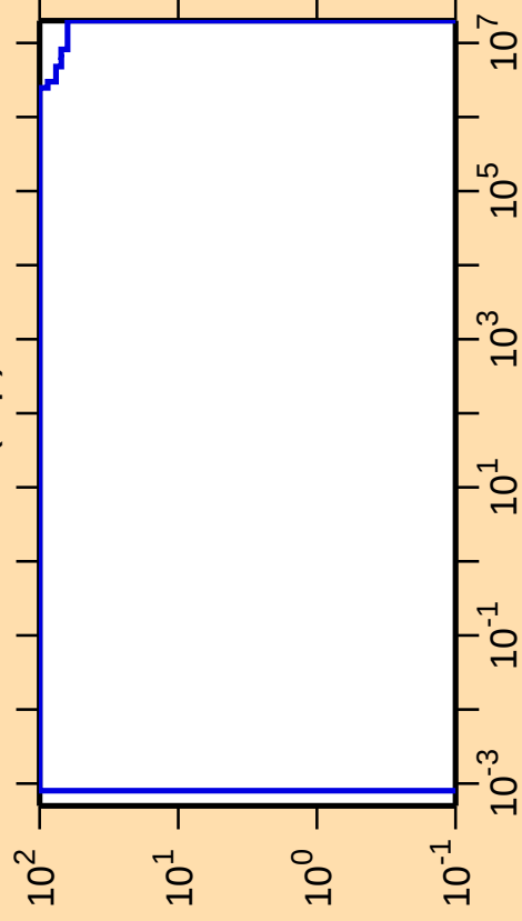
\Delta\sigma/\sigma vs. E for ^{184}\text{Pt}(n,p)
