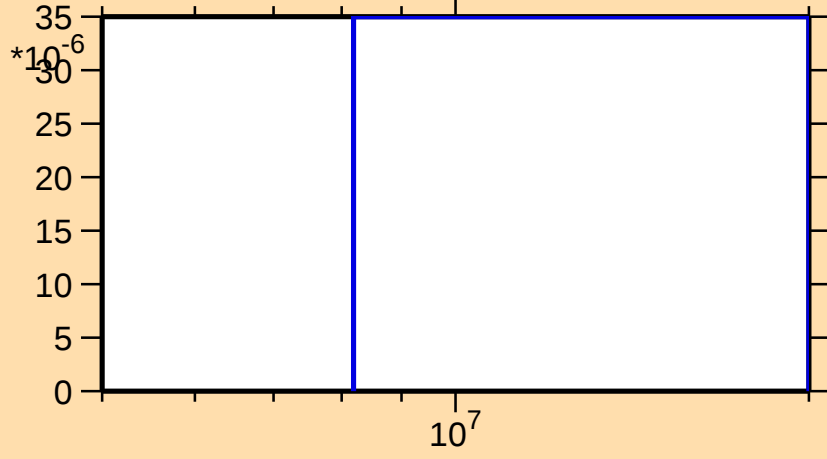
\sigma vs. E for ^{184}\text{Pt}(n,t)
