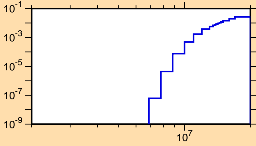
\sigma vs. E for ^{185}\text{Pt}(n,np)
