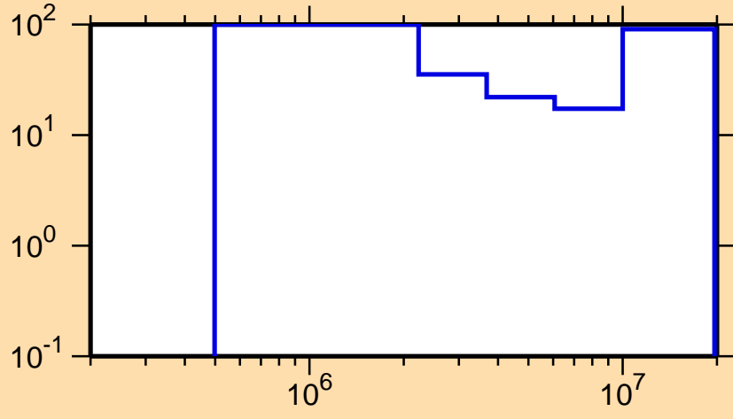
\Delta\sigma/\sigma vs. E for ^{185}\text{Pt}(n, ncont.)
