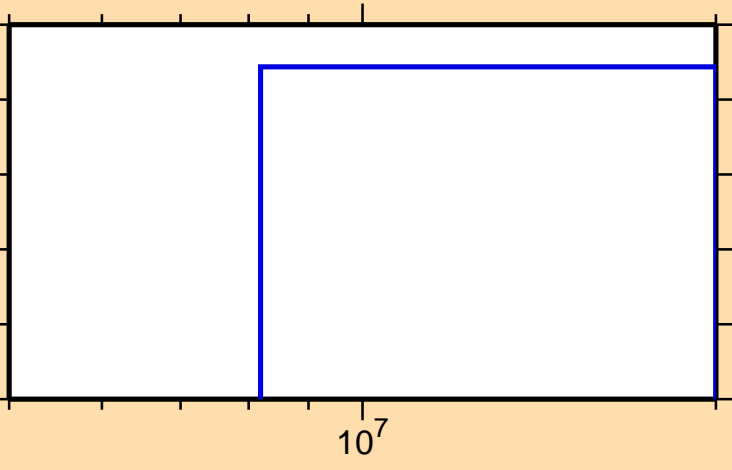
\sigma vs. E for ^{185}\text{Pt}(n,2np)
