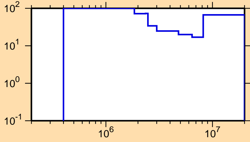
\Delta\sigma/\sigma vs. E for ^{185}\text{Pt}(n,n\text{cont.})
