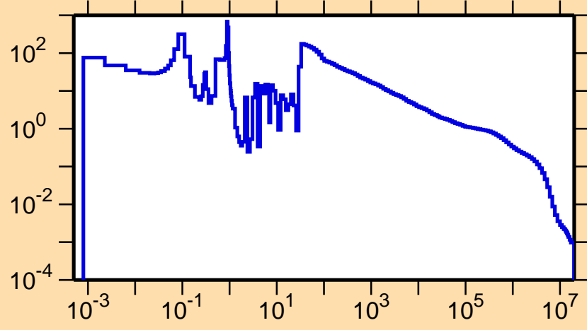
\sigma vs. E for ^{185}\text{Pt}(n,\gamma)
