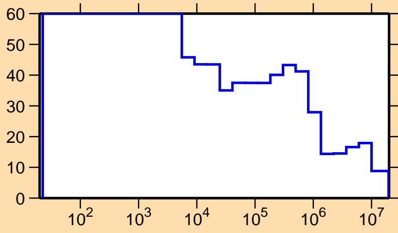
\Delta\sigma/\sigma vs. E for ^{185}\text{Pt}(n,\text{tot.})
