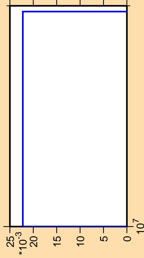
\Delta\sigma/\sigma vs. E for ^{185}\text{Pt}(n,3n\alpha)
