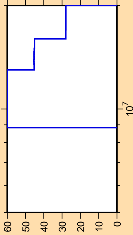
\Delta\sigma/\sigma vs. E for ^{186}\text{Pt}(n,2n)
