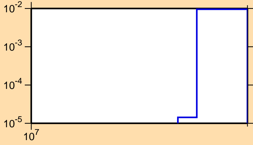
\sigma vs. E for ^{186}\text{Pt}(n,3n)
