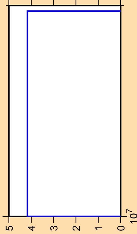
\Delta\sigma/\sigma vs. E for ^{186}\text{Pt}(\text{mt117})
