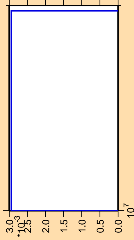
\Delta\sigma/\sigma vs. E for ^{186}\text{Pt}(n,3n\alpha)
