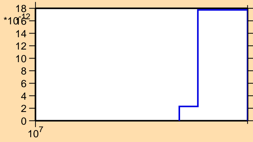
\sigma vs. E for ^{187}\text{Pt}(\text{mt117})
