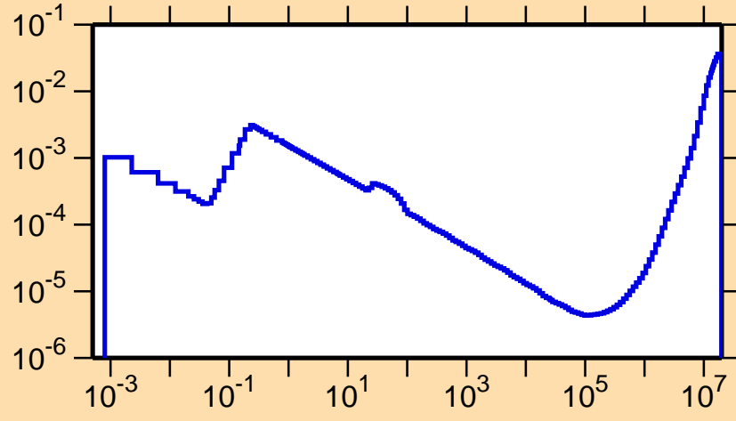
\sigma vs. E for ^{187}\text{Pt}(n,p)
