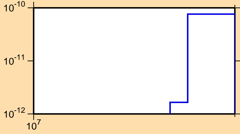
\sigma vs. E for ^{187}\text{Pt}(n,\text{pt})
