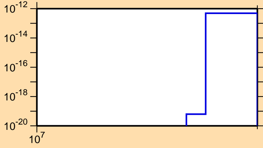
\sigma vs. E for ^{187}\text{Pt}(n,3n\alpha)
