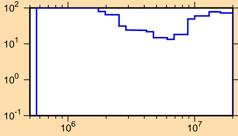
\Delta\sigma/\sigma vs. E for ^{187}\text{Pt}(n,ncont.)
