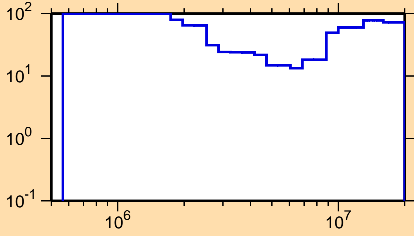
\Delta\sigma/\sigma vs. E for ^{187}\text{Pt}(n,n\text{cont.})
