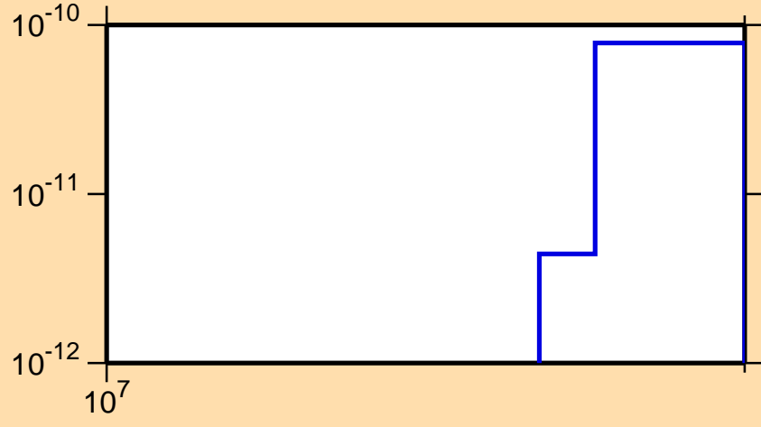
\sigma vs. E for ^{187}\text{Pt}(n,\text{pd})
