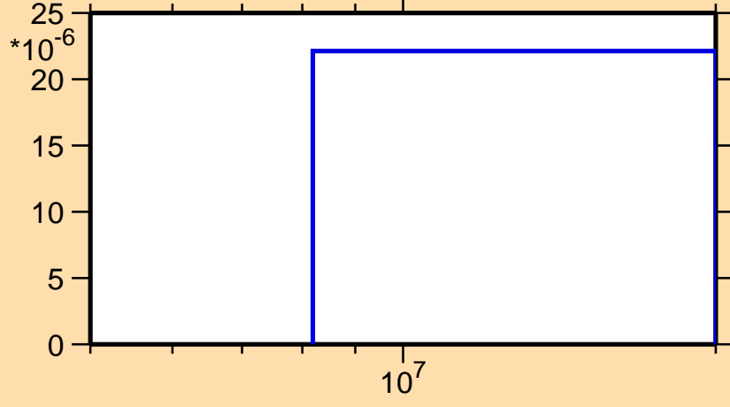
\sigma vs. E for ^{188}\text{Pt}(n,t)
