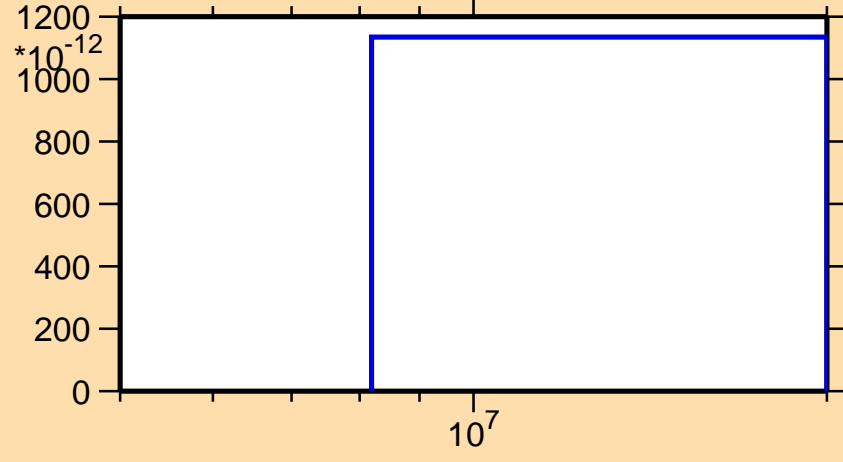
\sigma vs. E for ^{188}\text{Pt}(n,p\alpha)
