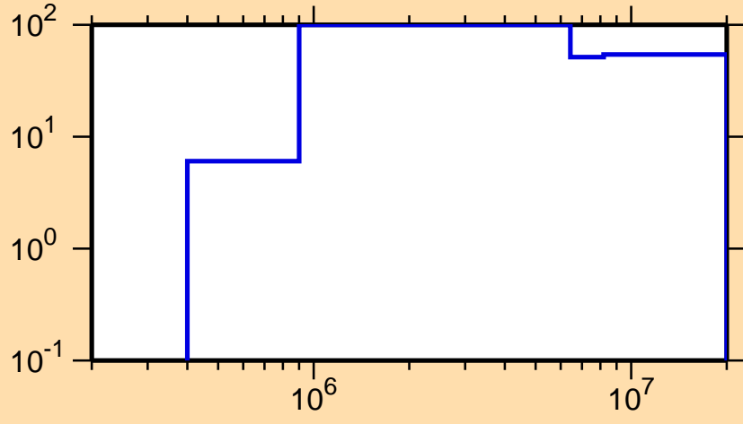
\Delta\sigma/\sigma vs. E for ^{188}\text{Pt}(n,p)
