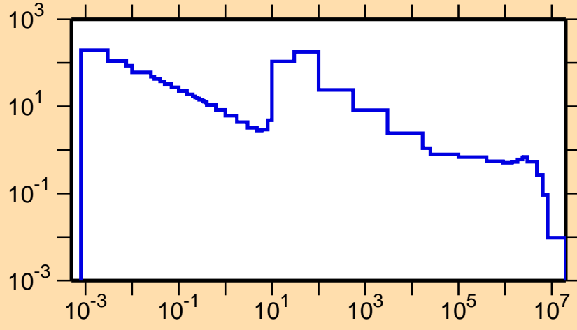
\sigma vs. E for ^{188}\text{Pt}(n,\gamma)
