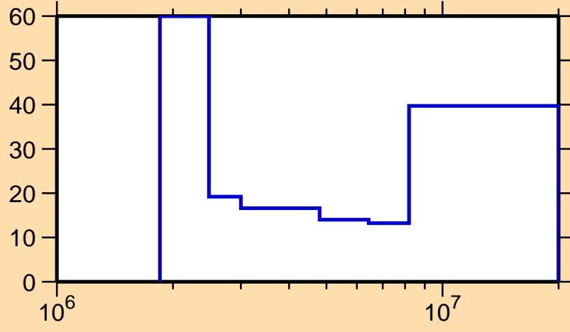
\Delta\sigma/\sigma vs. E for ^{188}\text{Pt}(n,n\text{cont.})
