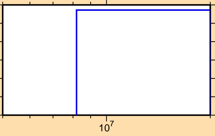
\sigma vs. E for ^{188}\text{Pt}(\text{mt } 34)
