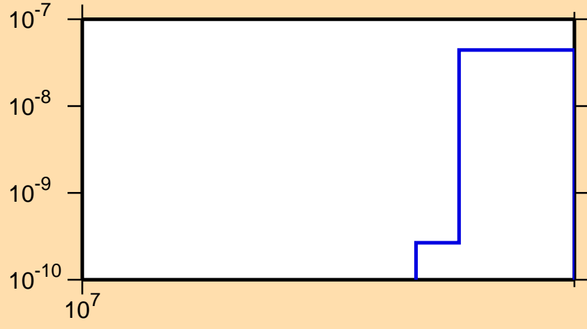
\sigma vs. E for ^{190}\text{Pt}(n,\text{nd})
