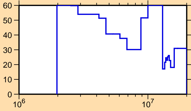
\Delta\sigma/\sigma vs. E for ^{190}\text{Pt}(n,n\text{cont.})
