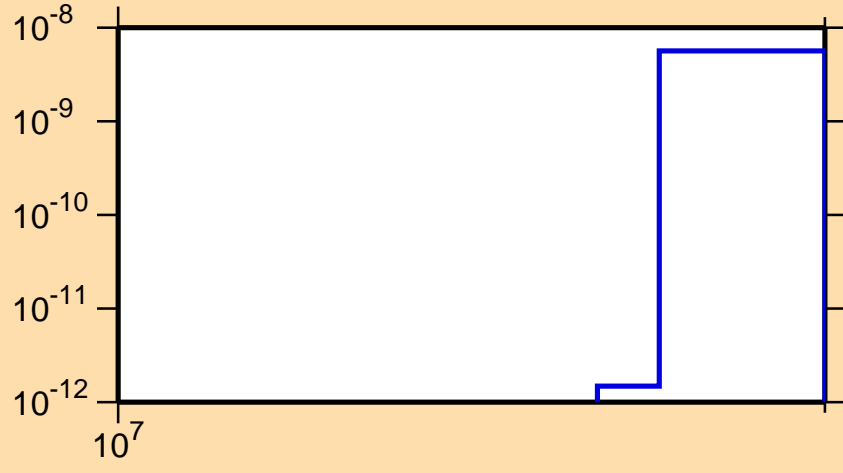
\sigma vs. E for ^{190}\text{Pt}(n,nt)
