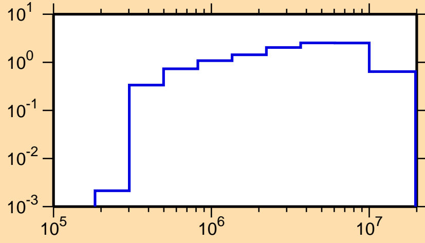
\sigma vs. E for ^{190}\text{Pt}(n,\text{inel.})
