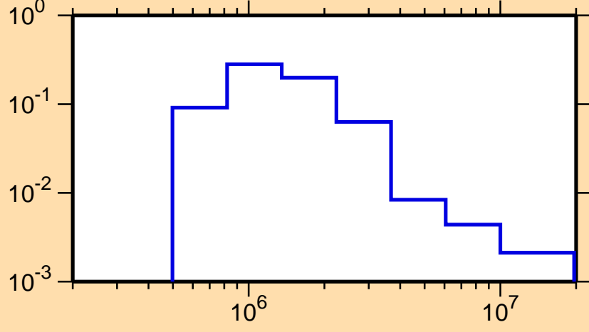
\sigma vs. E for ^{190}\text{Pt}(n,n_2)
