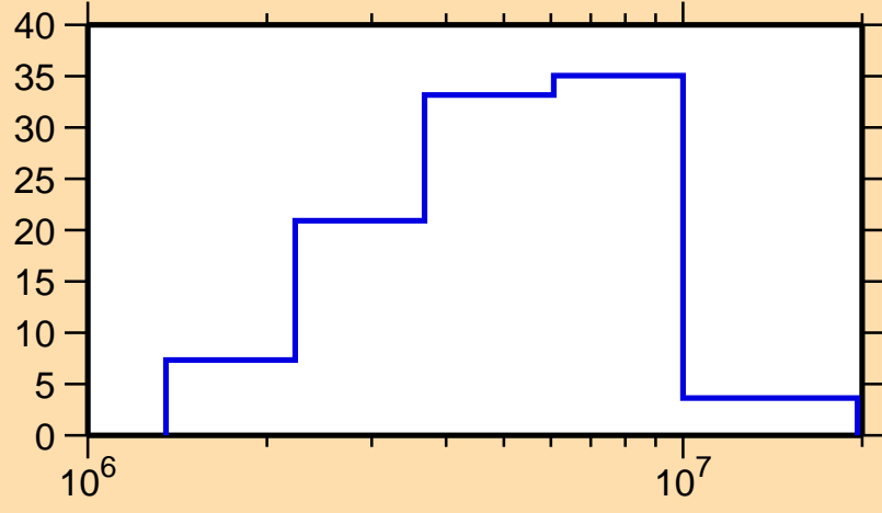
\Delta\sigma/\sigma vs. E for ^{190}\text{Pt}(n, el.)
