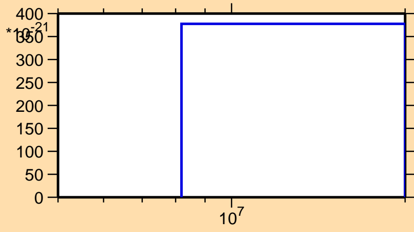
\sigma vs. E for ^{190}\text{Pt}(\text{mt } 11)
