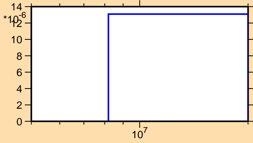
\sigma vs. E for ^{190}\text{Pt}(n,t)
