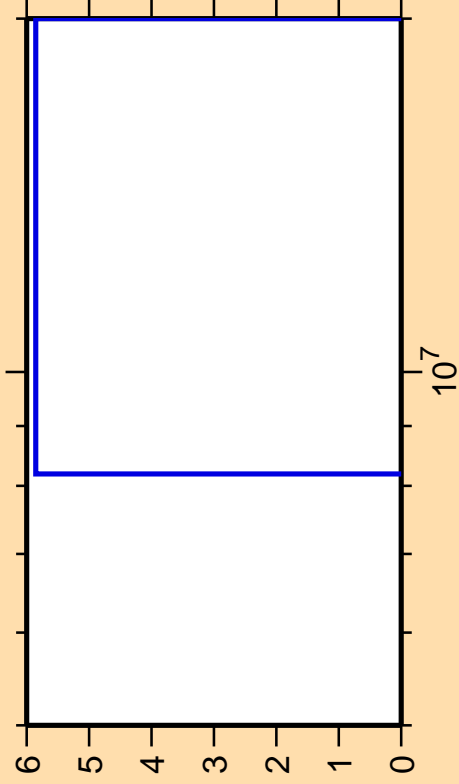
\Delta\sigma/\sigma vs. E for ^{190}\text{Pt}(n,t)
