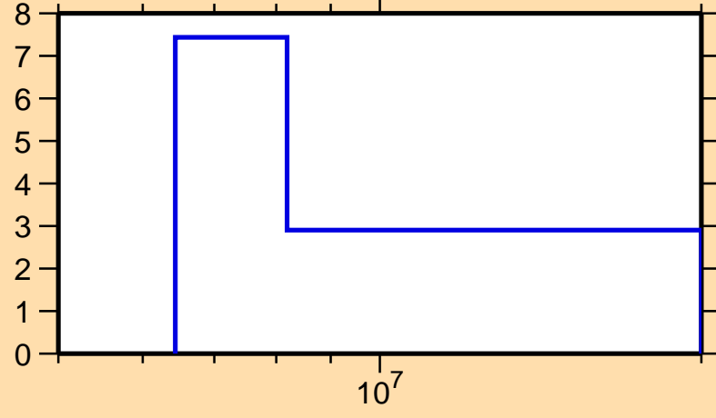
\Delta\sigma/\sigma vs. E for ^{191}\text{Pt}(n,\text{tot.})
