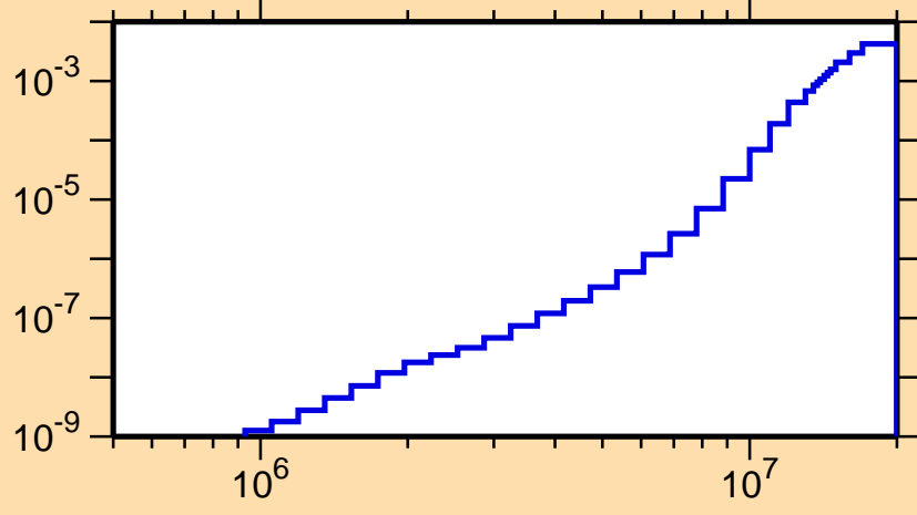
\sigma vs. E for ^{192}\text{Pt}(n,\alpha)
