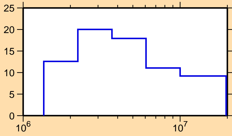
\Delta\sigma/\sigma vs. E for ^{192}\text{Pt}(n,n\text{nonel.})
