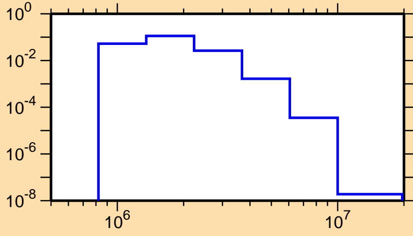
\sigma vs. E for ^{192}\text{Pt}(n,n_4)
