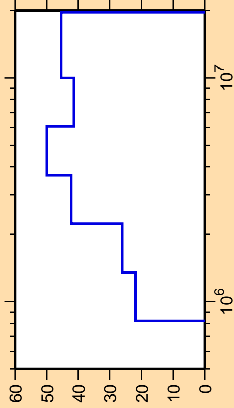
\Delta\sigma/\sigma vs. E for ^{192}\text{Pt}(n,n_4)
