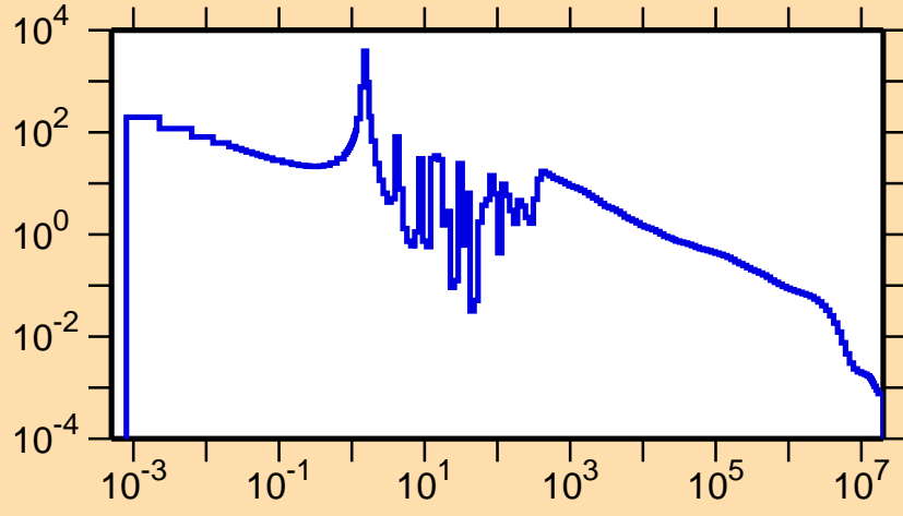
\sigma vs. E for ^{193}\text{Pt}(n,\gamma)
