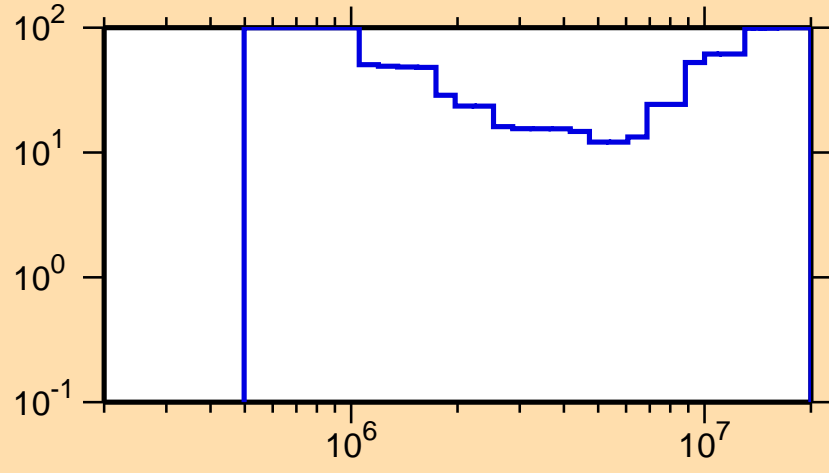
\Delta\sigma/\sigma vs. E for ^{193}\text{Pt}(n,n\text{cont.})
