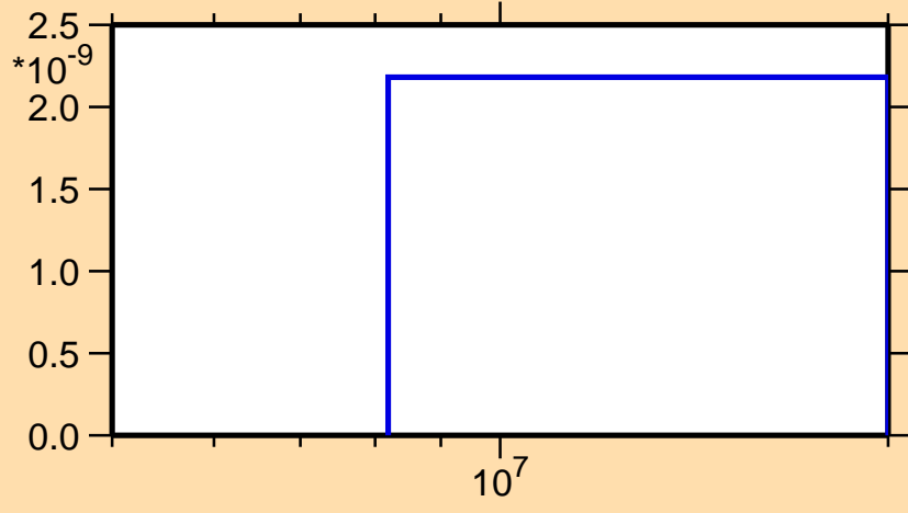
\sigma vs. E for ^{193}\text{Pt}(n,\text{nd})
