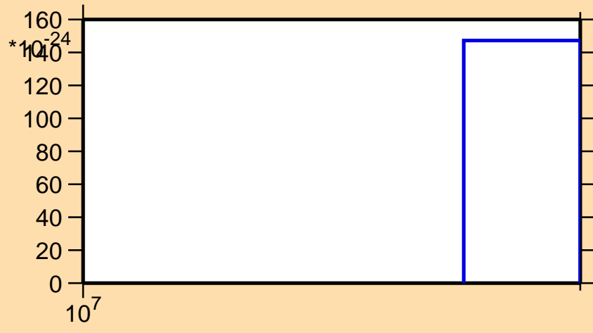
\sigma vs. E for ^{194}\text{Pt}(\text{mt } 11)
