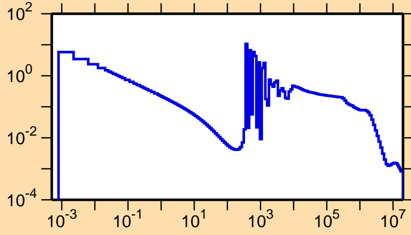
\sigma vs. E for ^{194}\text{Pt}(n,\gamma)
