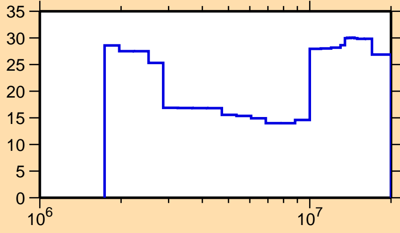
\Delta\sigma/\sigma vs. E for ^{194}\text{Pt}(n,n\text{cont.})
