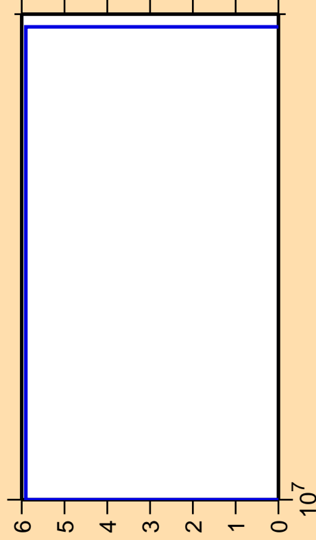
\Delta\sigma/\sigma vs. E for ^{194}\text{Pt}(n,2np)
