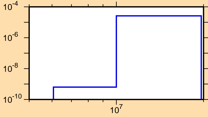
\sigma vs. E for ^{194}\text{Pt}(n,n\alpha)
