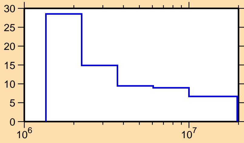
\Delta\sigma/\sigma vs. E for ^{194}\text{Pt}(n,n\text{onel.})
