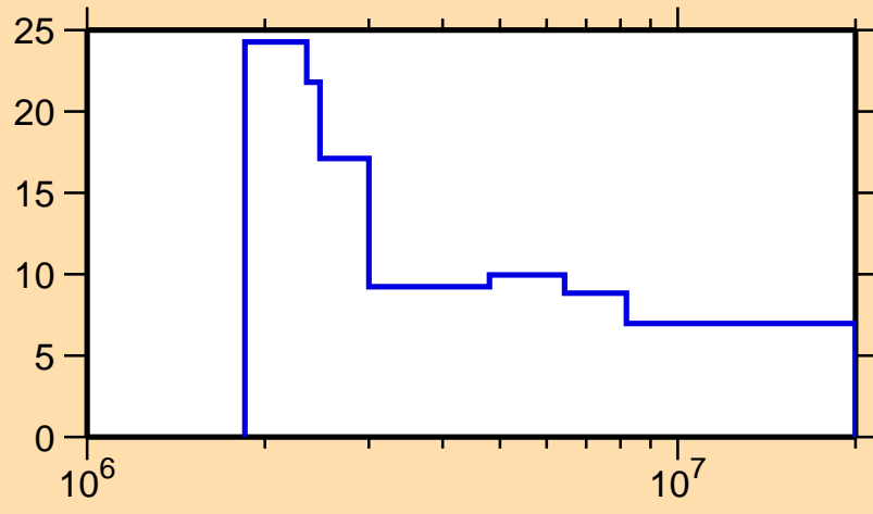
\Delta\sigma/\sigma vs. E for ^{194}\text{Pt}(n,n\text{oncl.})
