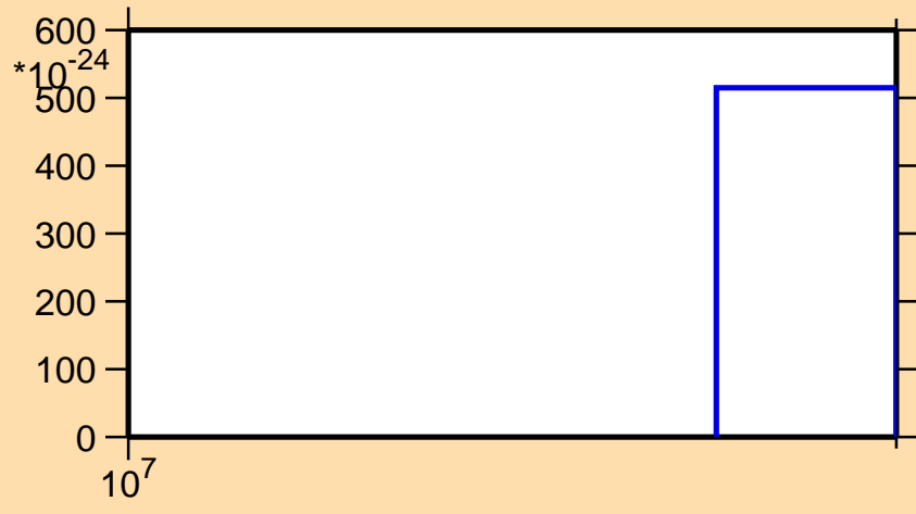
\sigma vs. E for ^{195}\text{Pt}(\text{mt } 11)
