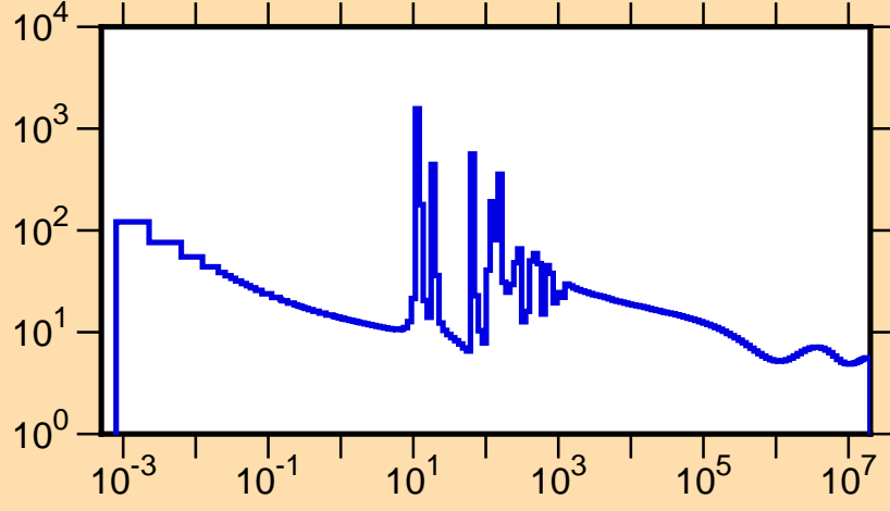
\sigma vs. E for ^{195}\text{Pt}(n,\text{tot.})
