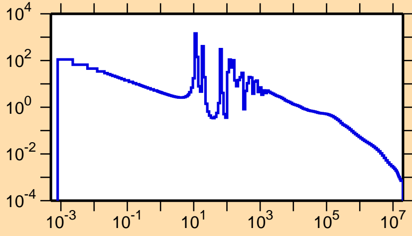
\sigma vs. E for ^{195}\text{Pt}(n,\gamma)
