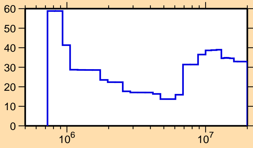
\Delta\sigma/\sigma vs. E for ^{195}\text{Pt}(n,ncont.)
