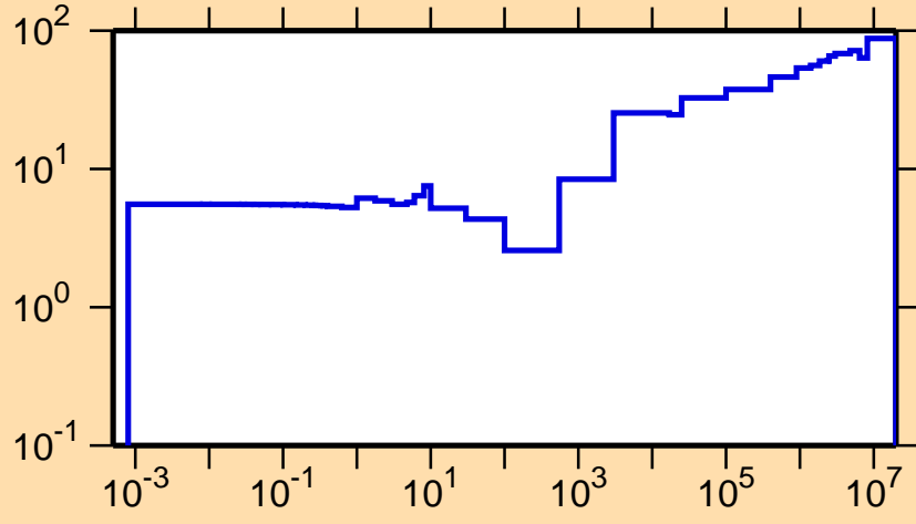
\Delta\sigma/\sigma vs. E for ^{195}\text{Pt}(n,\gamma)
