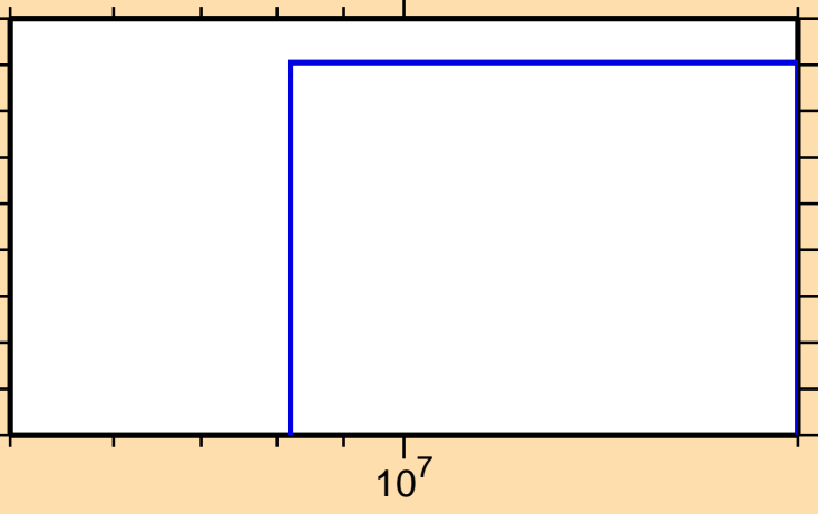
\sigma vs. E for ^{195}\text{Pt}(n,3n)
