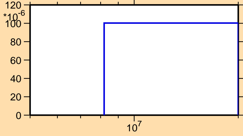
\sigma vs. E for ^{195}\text{Pt}(n,d)
