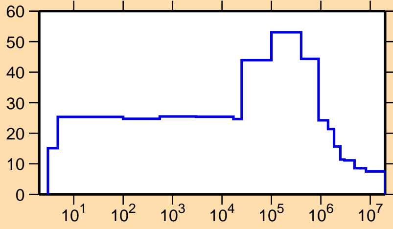
\Delta\sigma/\sigma vs. E for ^{195}\text{Pt}(n,\text{nonel.})
