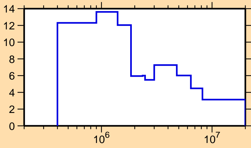
\Delta\sigma/\sigma vs. E for ^{195}\text{Pt}(n, \text{tot.})
