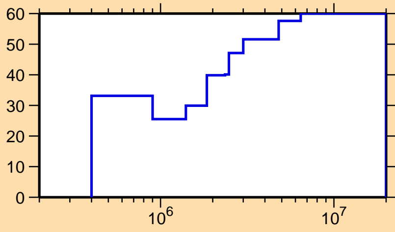
\Delta\sigma/\sigma vs. E for ^{195}\text{Pt}(n,n_1)
