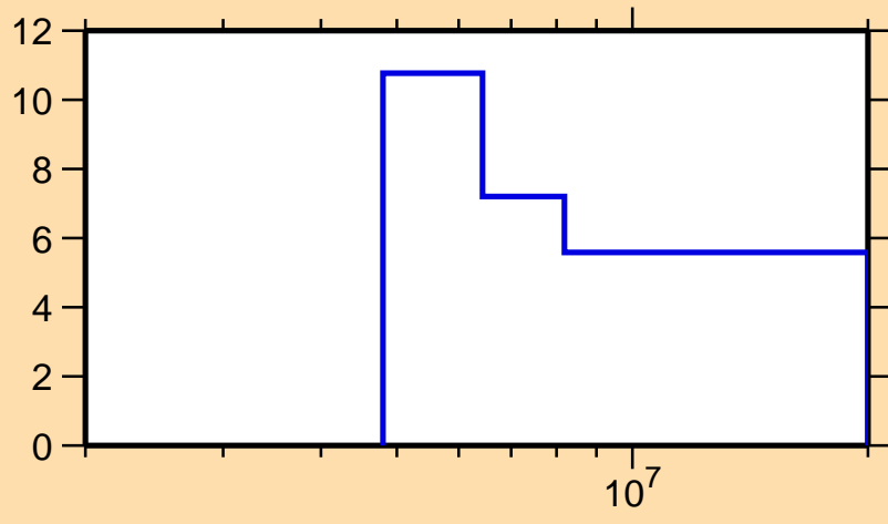
\Delta\sigma/\sigma vs. E for ^{195}\text{Pt}(n,\text{el.})
