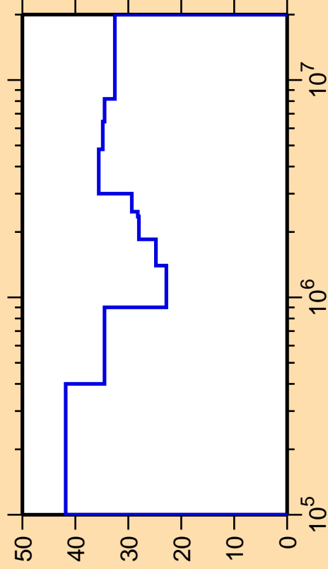
\Delta\sigma/\sigma vs. E for ^{195}\text{Pt}(n,n_4)
