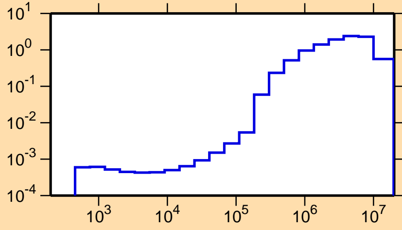
\sigma vs. E for ^{195}\text{Pt}(n,\text{inel.})
