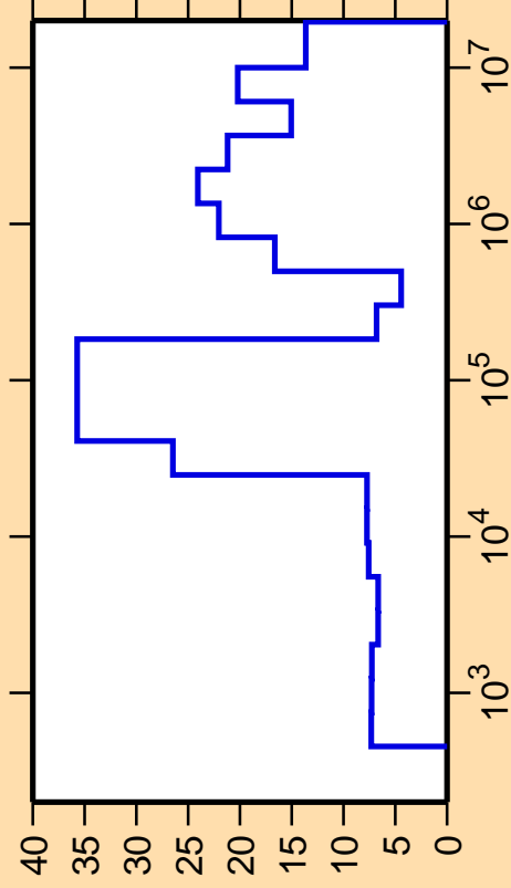
\Delta\sigma/\sigma vs. E for ^{195}\text{Pt}(n,\text{inel.})
