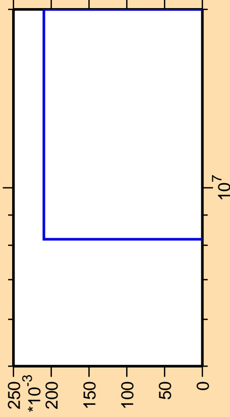
\Delta\sigma/\sigma vs. E for ^{195}\text{Pt}(n,\text{He3})
