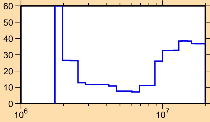
\Delta\sigma/\sigma vs. E for ^{196}\text{Pt}(n,n\text{cont.})
