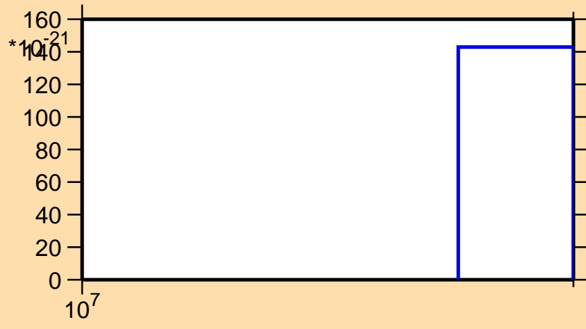
\sigma vs. E for ^{196}\text{Pt}(\text{mt } 11)
