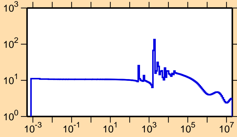
\sigma vs. E for ^{196}\text{Pt}(n,\text{el.})
