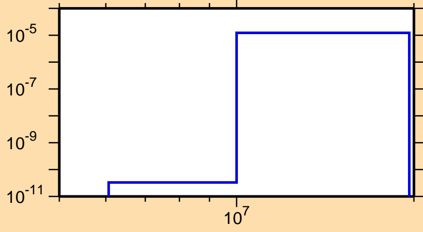
\sigma vs. E for ^{196}\text{Pt}(n,n\alpha)
