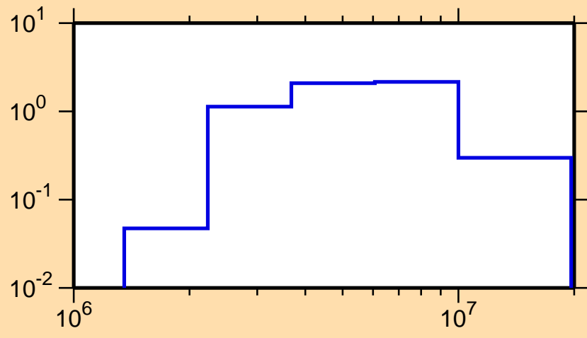
\sigma vs. E for ^{196}\text{Pt}(n,n\text{cont.})
