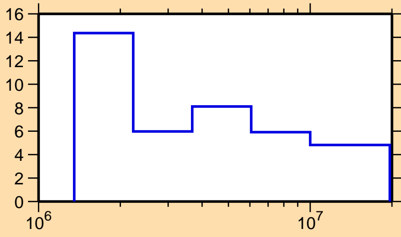
\Delta\sigma/\sigma vs. E for ^{196}\text{Pt}(n,n\text{onel.})
