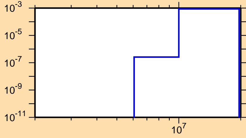
\sigma vs. E for ^{196}\text{Pt}(n,p)
