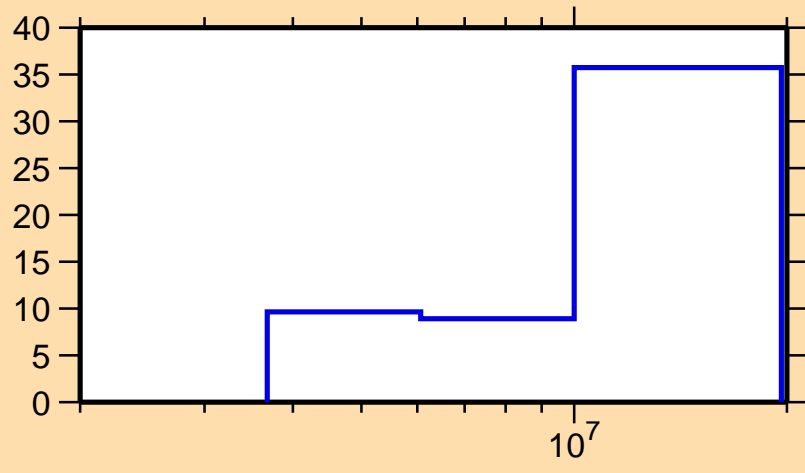
\Delta\sigma/\sigma vs. E for ^{196}\text{Pt}(n,ncont.)
