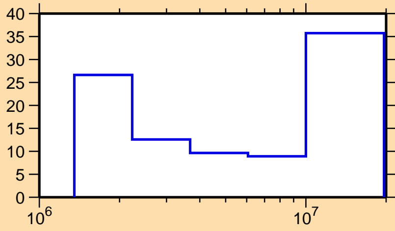
\Delta\sigma/\sigma vs. E for ^{196}\text{Pt}(n,n\text{cont.})
