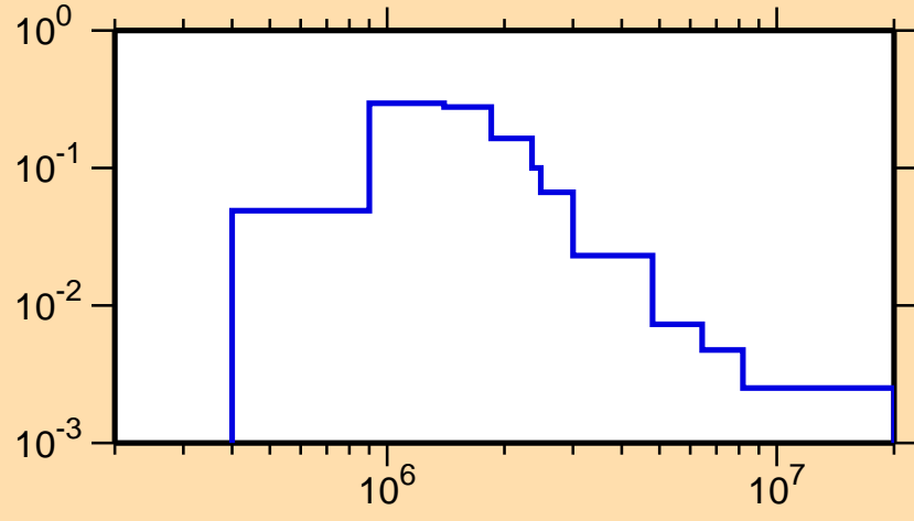
\sigma vs. E for ^{196}\text{Pt}(n,n_2)
