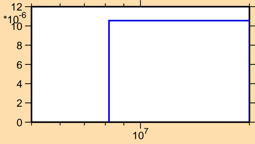
\sigma vs. E for ^{196}\text{Pt}(n,np)
