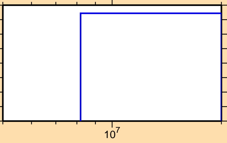
\sigma vs. E for ^{196}\text{Pt}(n,d)
