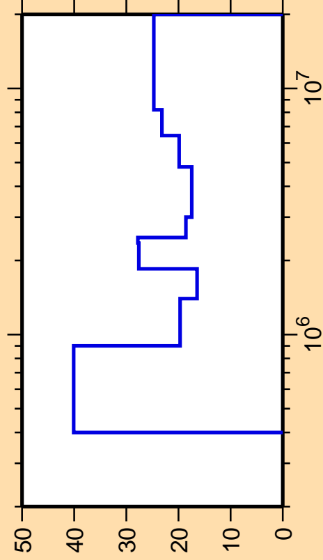
\Delta\sigma/\sigma vs. E for ^{196}\text{Pt}(n,n_2)
