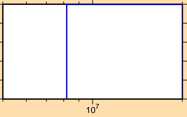
\sigma vs. E for ^{197}\text{Pt}(n,\text{nd})
