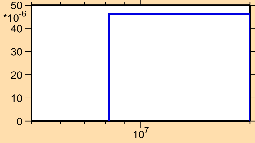
\sigma vs. E for ^{197}\text{Pt}(n,d)
