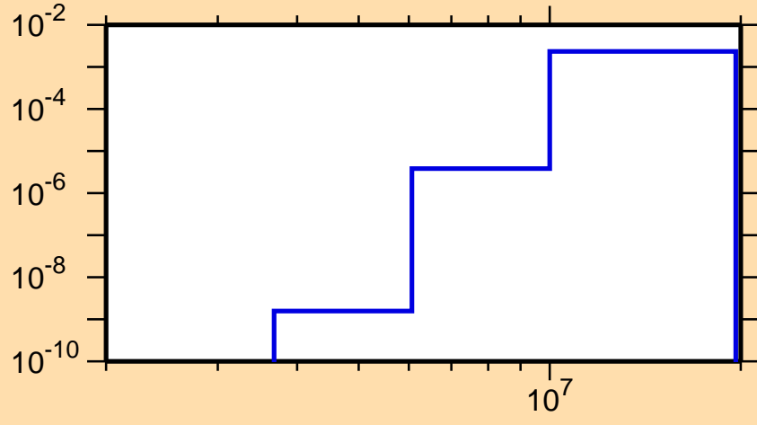
\sigma vs. E for ^{197}\text{Pt}(n,p)
