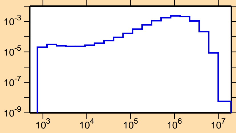
\sigma vs. E for ^{197}\text{Pt}(n,n_3)
