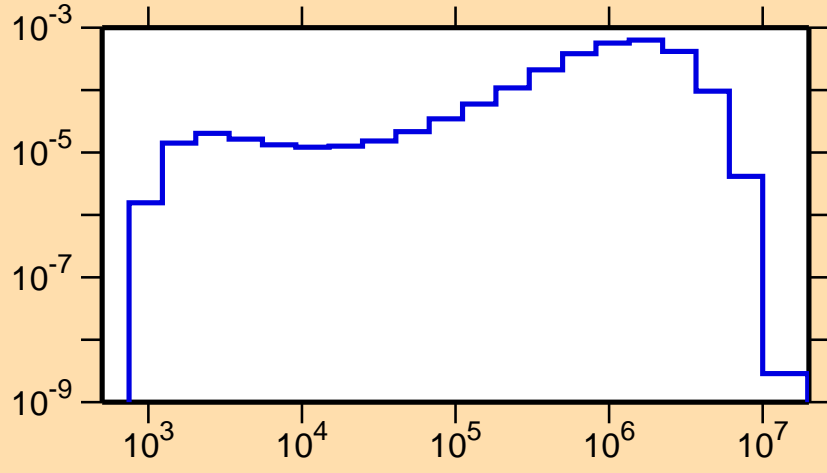
\sigma vs. E for ^{197}\text{Pt}(n,n_1)
