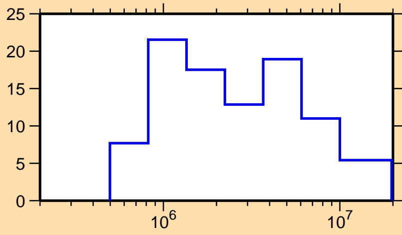
\Delta\sigma/\sigma vs. E for ^{197}\text{Pt}(n, el.)
