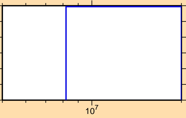
\sigma vs. E for ^{197}\text{Pt}(n,3n)
