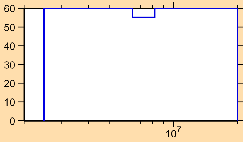
\Delta\sigma/\sigma vs. E for ^{197}\text{Pt}(n,\gamma)
