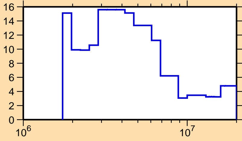
\Delta\sigma/\sigma vs. E for ^{198}\text{Pt}(n,tot.)
