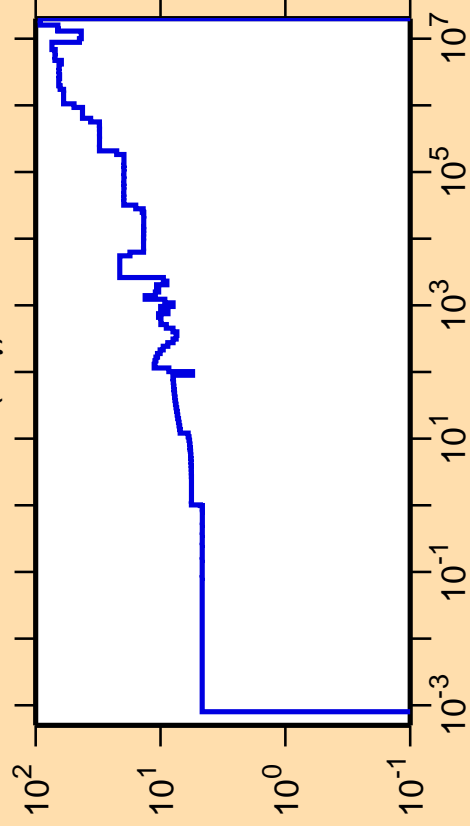
\Delta\sigma/\sigma vs. E for ^{198}\text{Pt}(n,\gamma)
