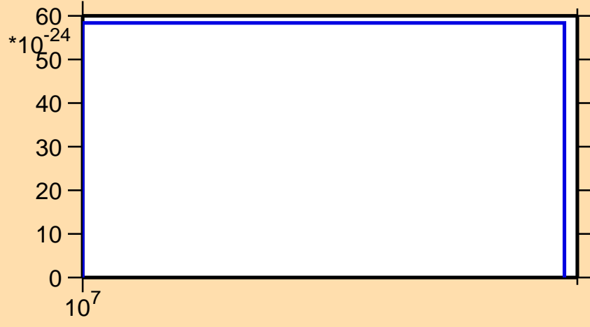
\sigma vs. E for ^{198}\text{Pt}(\text{mt } 11)
