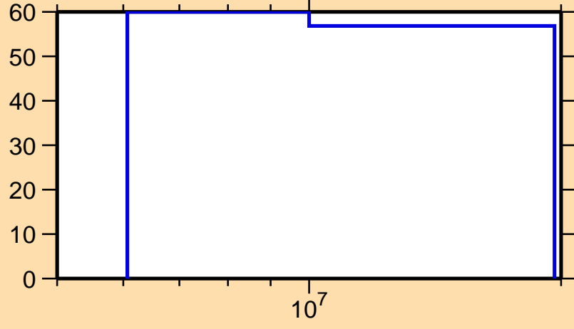
\Delta\sigma/\sigma vs. E for ^{198}\text{Pt}(n,p)
