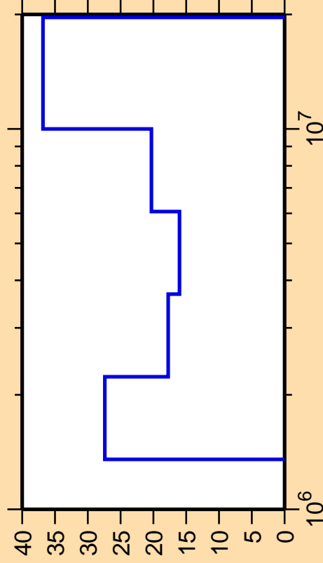
\Delta\sigma/\sigma vs. E for ^{198}\text{Pt}(n,n\text{cont.})
