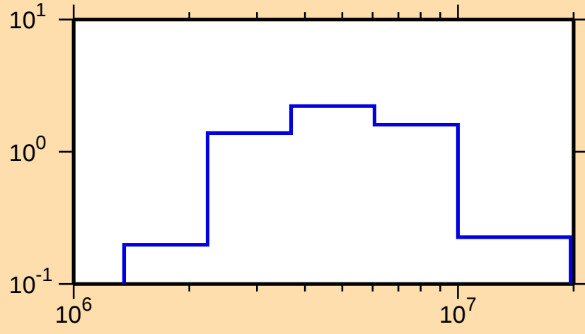
\sigma vs. E for ^{199}\text{Pt}(n,n\text{cont.})
