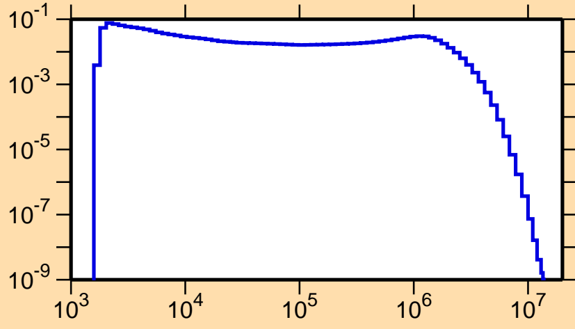
\sigma vs. E for ^{199}\text{Pt}(n,n_1)
