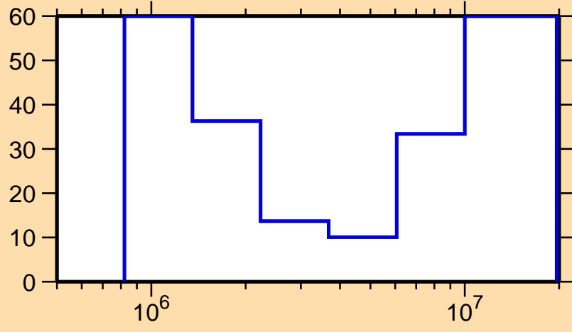
\Delta\sigma/\sigma vs. E for ^{199}\text{Pt}(n,n\text{cont.})
