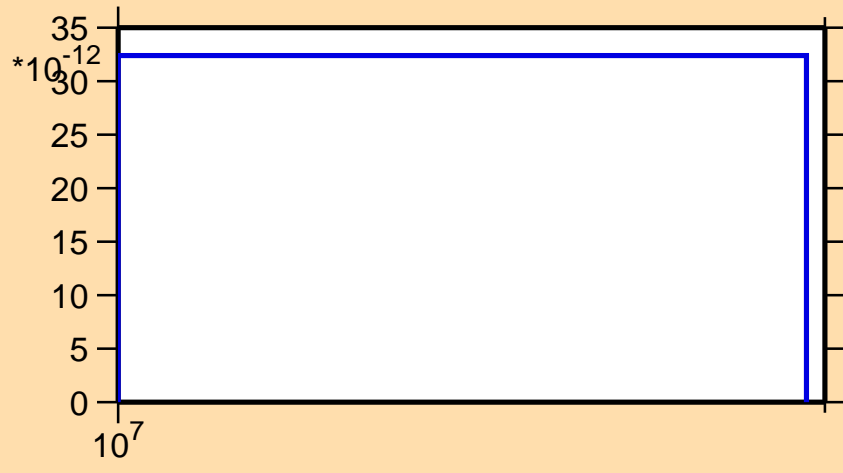
\sigma vs. E for ^{199}\text{Pt}(n,2np)
