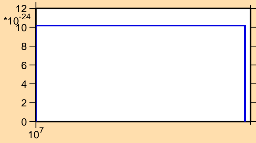
\sigma vs. E for ^{199}\text{Pt}(\text{mt } 11)
