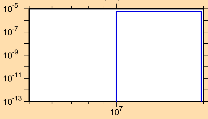
\sigma vs. E for ^{199}\text{Pt}(n,t)
