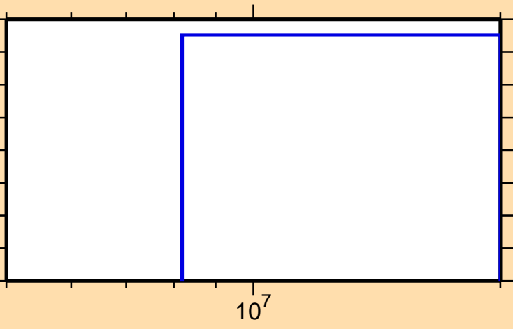
\sigma vs. E for ^{199}\text{Pt}(n,2np)
