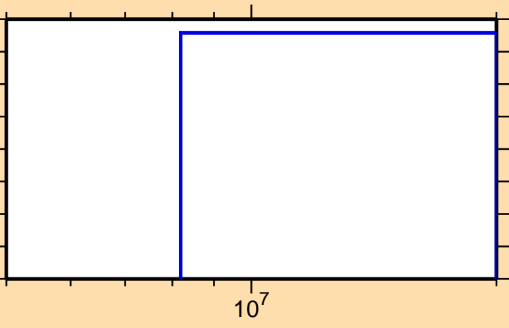
\sigma vs. E for ^{199}\text{Pt}(n,2n\alpha)
