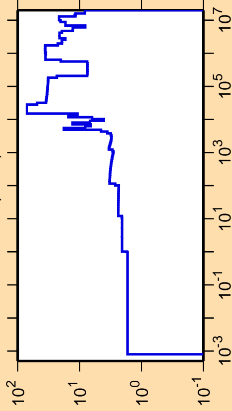
\Delta\sigma/\sigma vs. E for ^{200}\text{Pt}(n,\text{el.})
