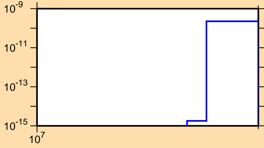
\sigma vs. E for ^{200}\text{Pt}(n,\text{nd})
