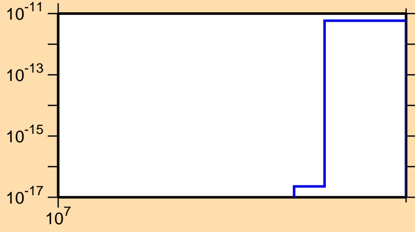
\sigma vs. E for ^{200}\text{Pt}(n,2np)
