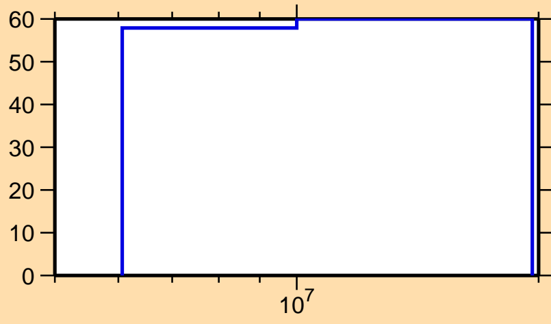
\Delta\sigma/\sigma vs. E for ^{200}\text{Pt}(n,p)
