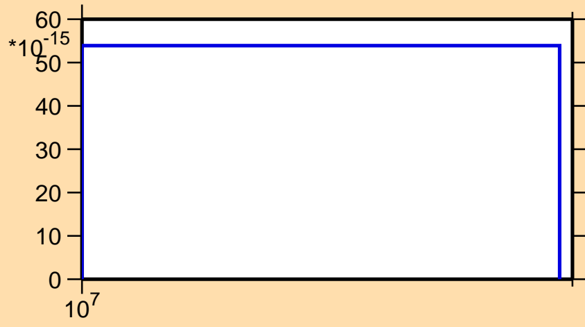
\sigma vs. E for ^{200}\text{Pt}(n,2n\alpha)
