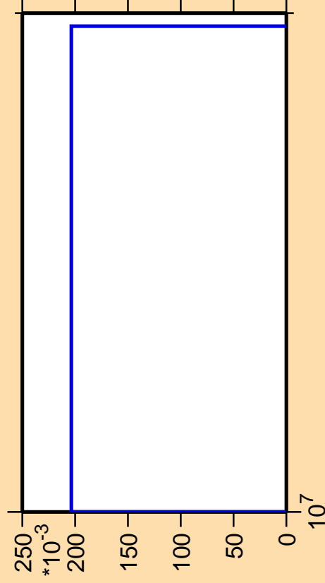
\Delta\sigma/\sigma vs. E for ^{200}\text{Pt}(n,2n\alpha)
