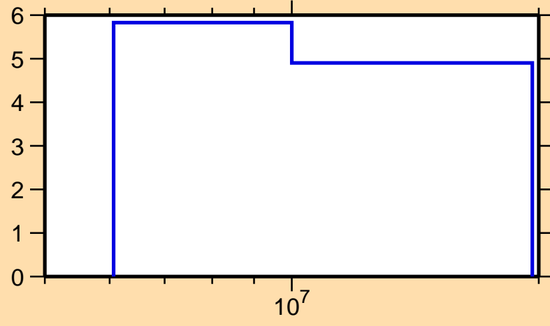
\Delta\sigma/\sigma vs. E for ^{200}\text{Pt}(n,\text{tot.})
