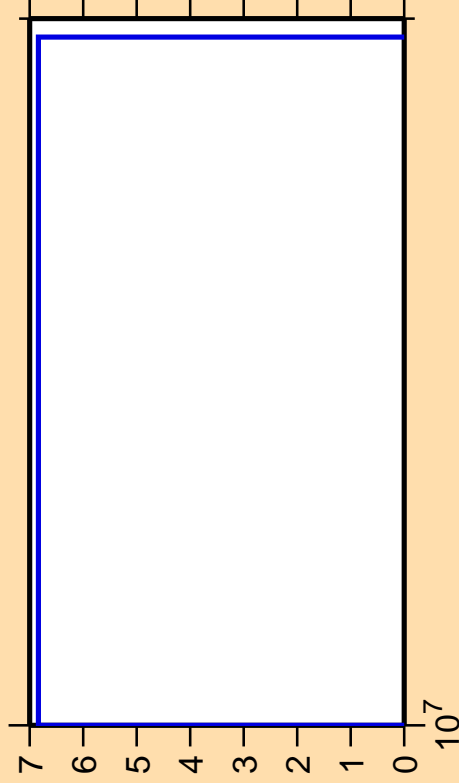
\Delta\sigma/\sigma vs. E for ^{200}\text{Pt}(n,\text{nd})
