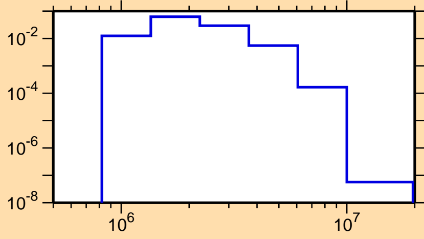
\sigma vs. E for ^{200}\text{Pt}(n,n_4)
