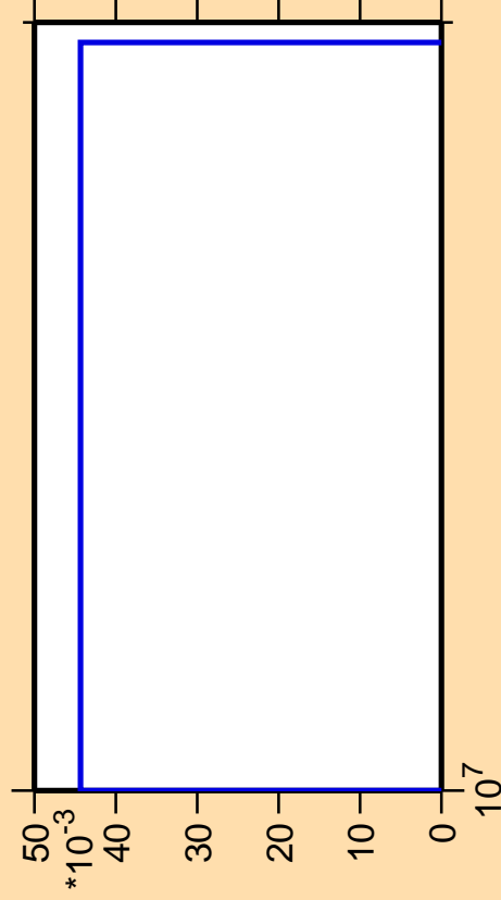
\Delta\sigma/\sigma vs. E for ^{200}\text{Pt}(n,2np)
