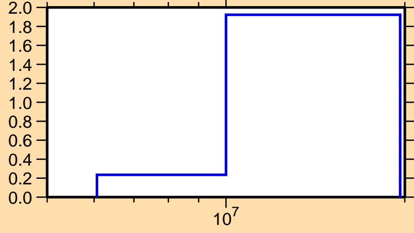
\sigma vs. E for ^{200}\text{Pt}(n,2n)
