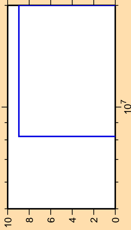
\Delta\sigma/\sigma vs. E for ^{200}\text{Pt}(n,nd)
