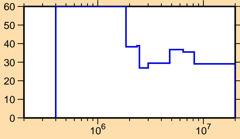
\Delta\sigma/\sigma vs. E for ^{200}\text{Pt}(n,n_1)
