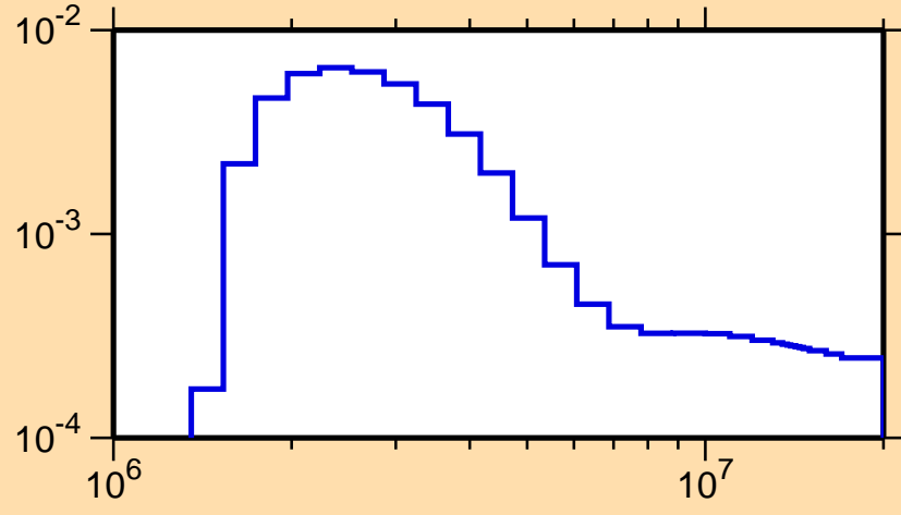
\sigma vs. E for ^{201}\text{Pt}(n,n_3)
