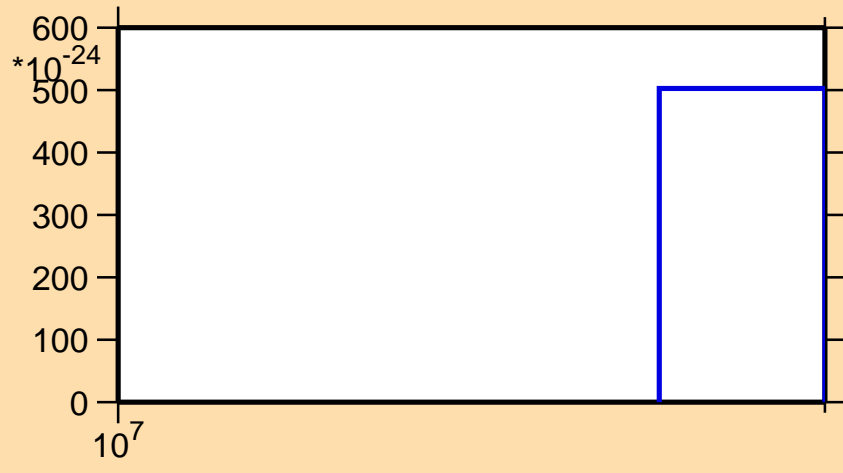
\sigma vs. E for ^{201}\text{Pt}(\text{mt } 11)
