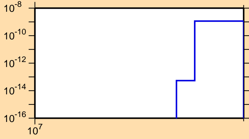
\sigma vs. E for ^{201}\text{Pt}(n,2np)
