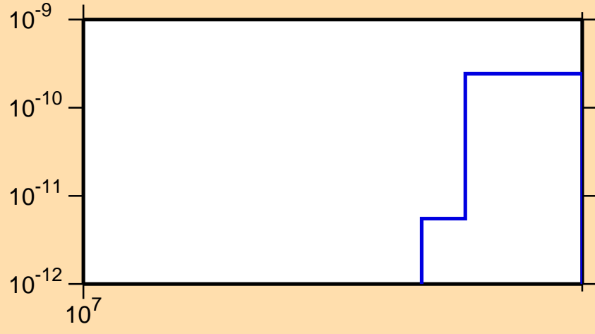
\sigma vs. E for ^{201}\text{Pt}(n,2n\alpha)
