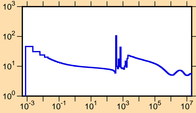
\sigma vs. E for ^{201}\text{Pt}(n,\text{tot.})
