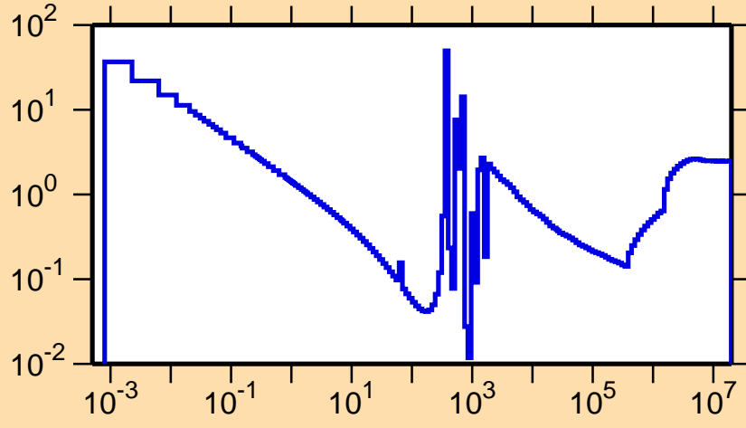
\sigma vs. E for ^{201}\text{Pt}(n,\text{nonel.})
