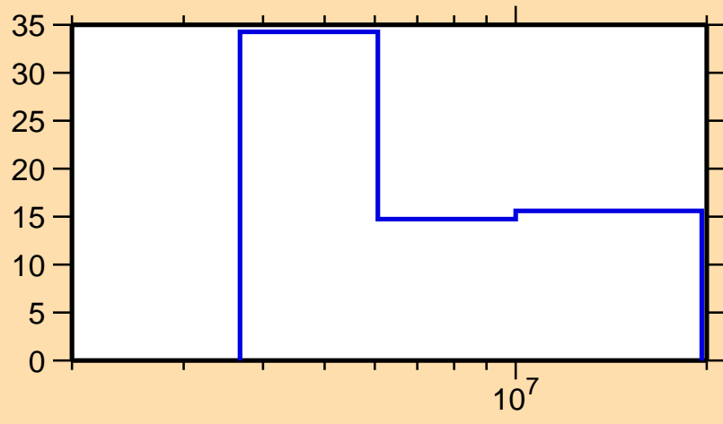
\Delta\sigma/\sigma vs. E for ^{201}\text{Pt}(n,2n)
