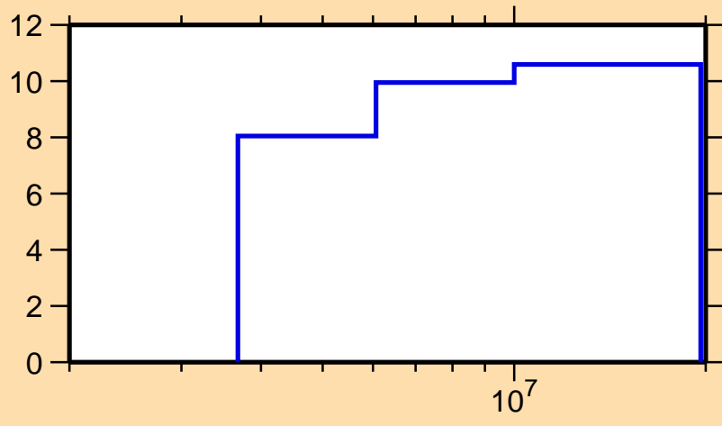
\Delta\sigma/\sigma vs. E for ^{201}\text{Pt}(n,n_1)
