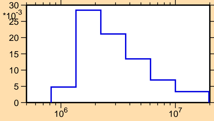
\sigma vs. E for ^{201}\text{Pt}(n,n_2)
