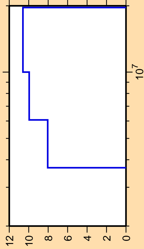
\Delta\sigma/\sigma vs. E for ^{201}\text{Pt}(n,n_1)
