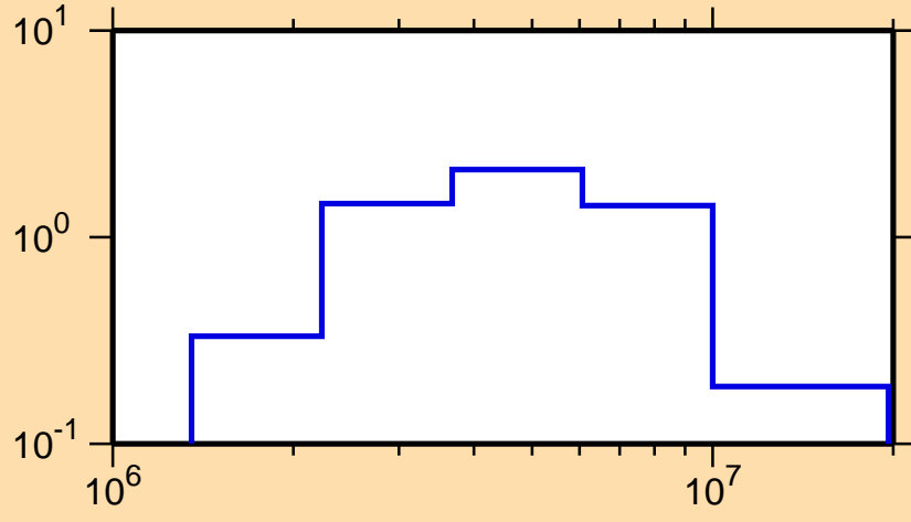
\sigma vs. E for ^{201}\text{Pt}(n,n\text{cont.})
