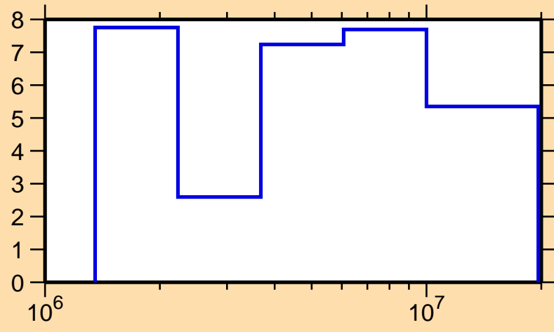
\Delta\sigma/\sigma vs. E for ^{201}\text{Pt}(n, \text{el.})
