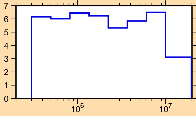
\Delta\sigma/\sigma vs. E for ^{201}\text{Pt}(n,\text{tot.})
