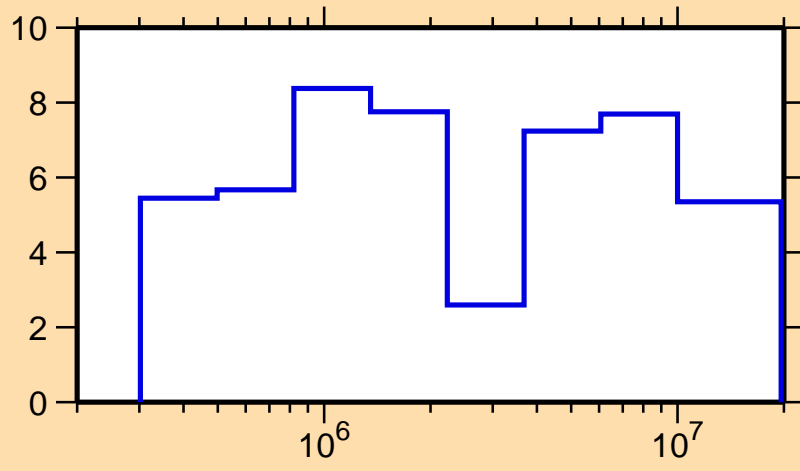
\Delta\sigma/\sigma vs. E for ^{201}\text{Pt}(n,\text{el.})
