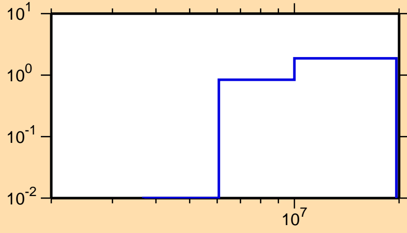
\sigma vs. E for ^{201}\text{Pt}(n,2n)
