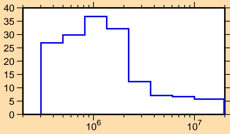
\Delta\sigma/\sigma vs. E for ^{201}\text{Pt}(n,\text{nonel.})
