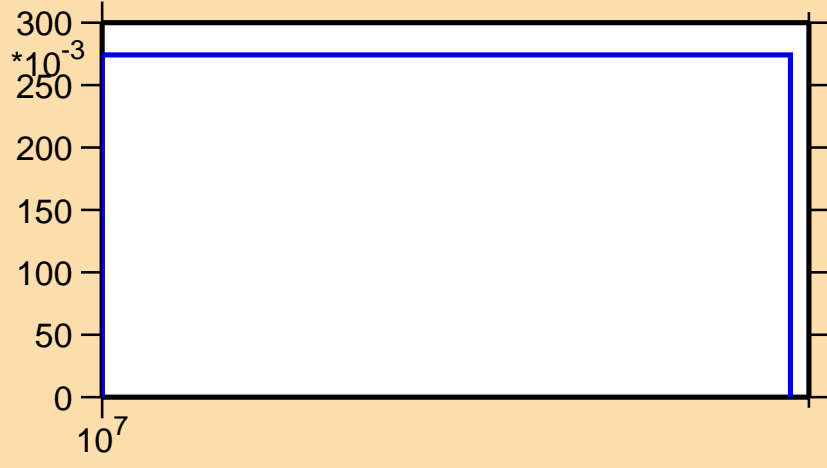
\sigma vs. E for ^{201}\text{Pt}(n,3n)
