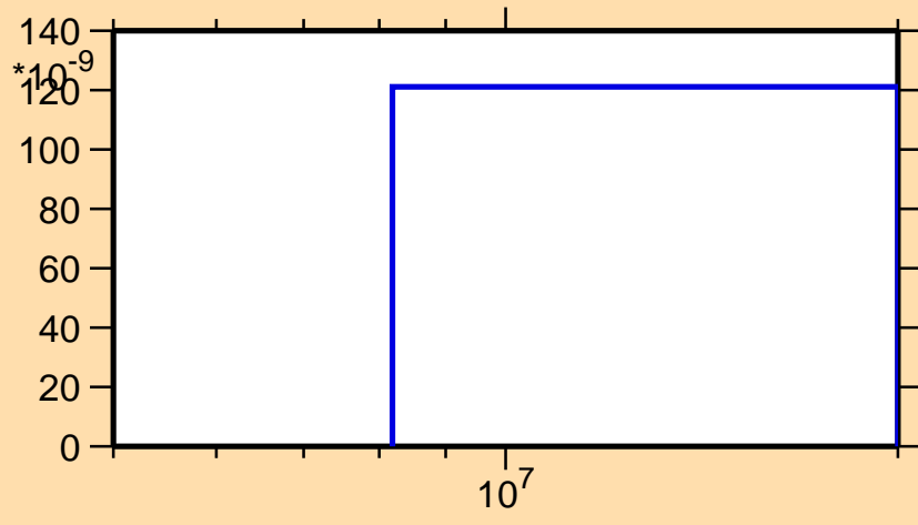
\sigma vs. E for ^{201}\text{Pt}(n,n\alpha)
