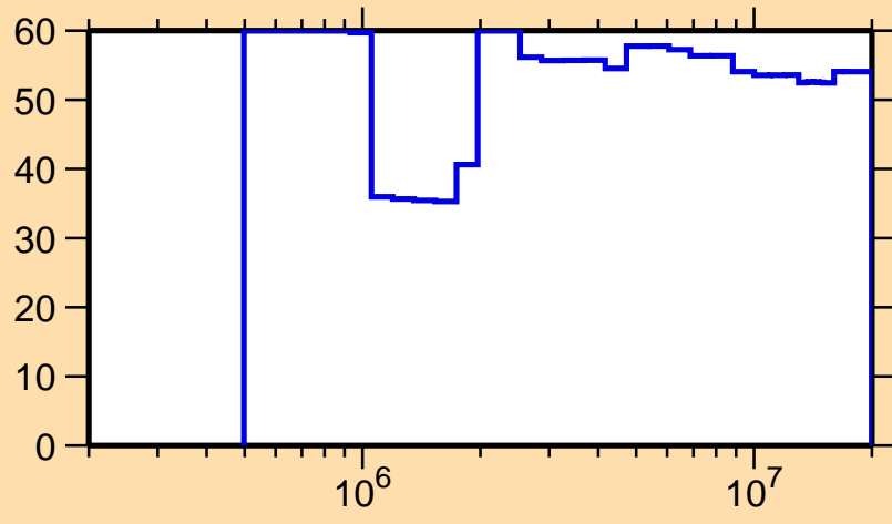
\Delta\sigma/\sigma vs. E for ^{202}\text{Pt}(n,n_1)
