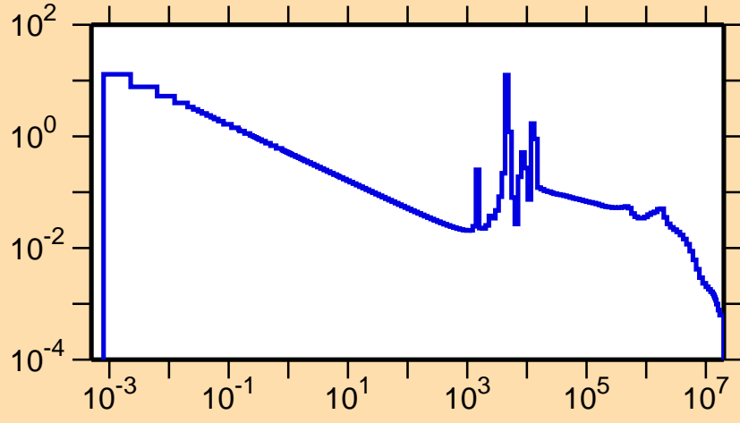
\sigma vs. E for ^{202}\text{Pt}(n,\gamma)
