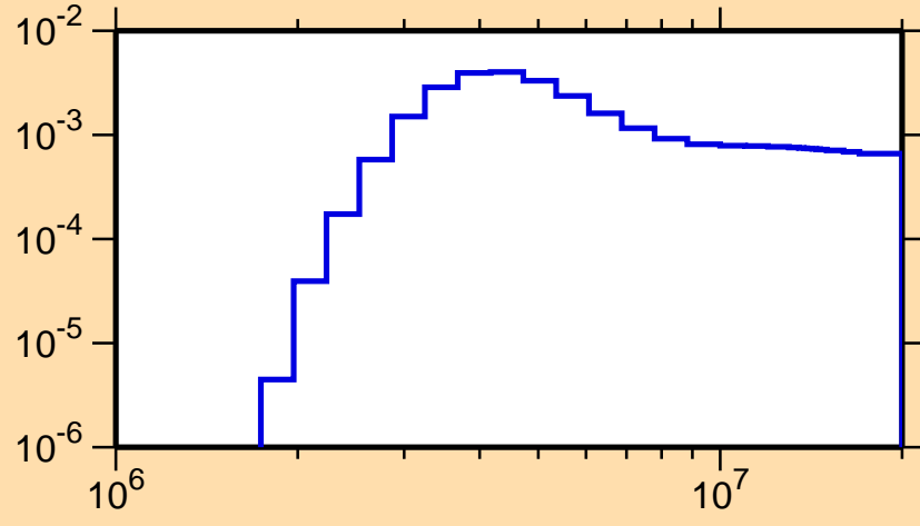
\sigma vs. E for ^{202}\text{Pt}(n,n_4)
