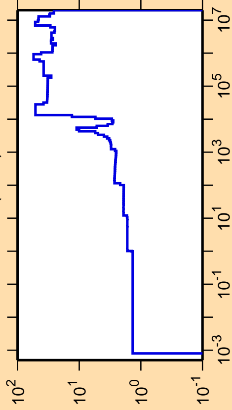
\Delta\sigma/\sigma vs. E for ^{202}\text{Pt}(n,\text{el.})
