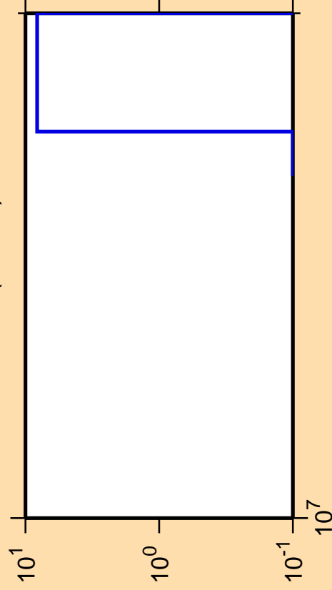
\Delta\sigma/\sigma vs. E for ^{202}\text{Pt}(n,2n\alpha)
