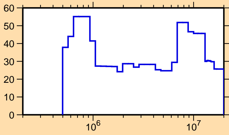
\Delta\sigma/\sigma vs. E for ^{202}\text{Pt}(n,\text{el.})
