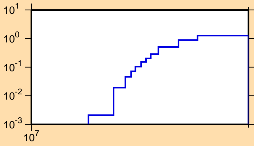
\sigma vs. E for ^{202}\text{Pt}(n,3n)
