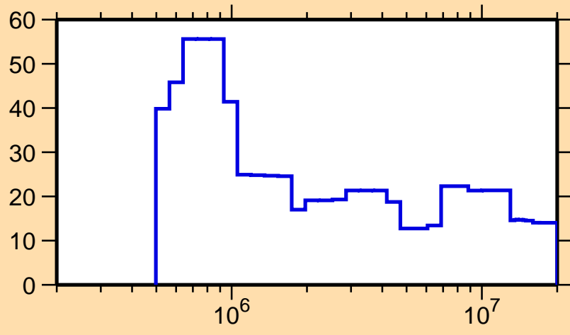
\Delta\sigma/\sigma vs. E for ^{202}\text{Pt}(n,\text{tot.})
