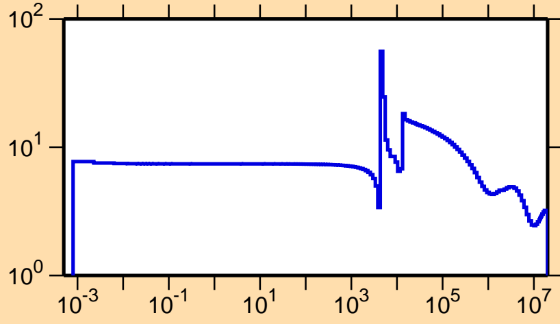
\sigma vs. E for ^{202}\text{Pt}(n,\text{el.})
