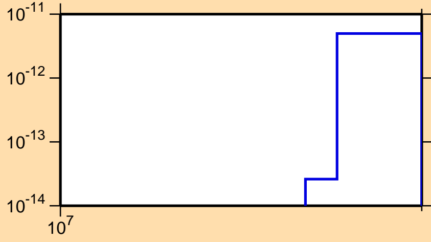
\sigma vs. E for ^{202}\text{Pt}(n,2n\alpha)
