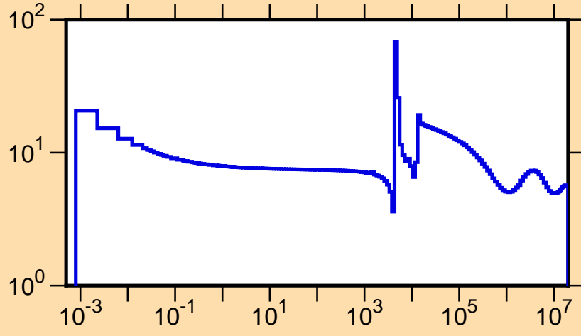
\sigma vs. E for ^{202}\text{Pt}(n,\text{tot.})
