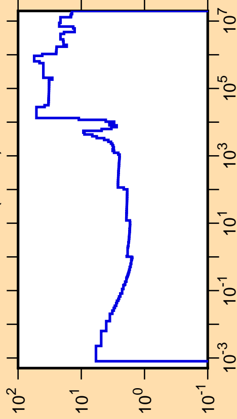
\Delta\sigma/\sigma vs. E for ^{202}\text{Pt}(n,\text{tot.})
