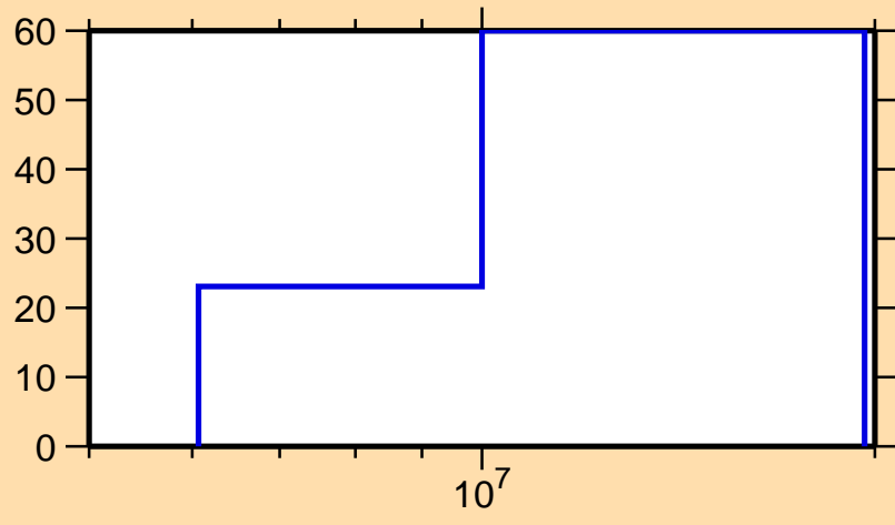
\Delta\sigma/\sigma vs. E for ^{202}\text{Pt}(n,ncont.)
