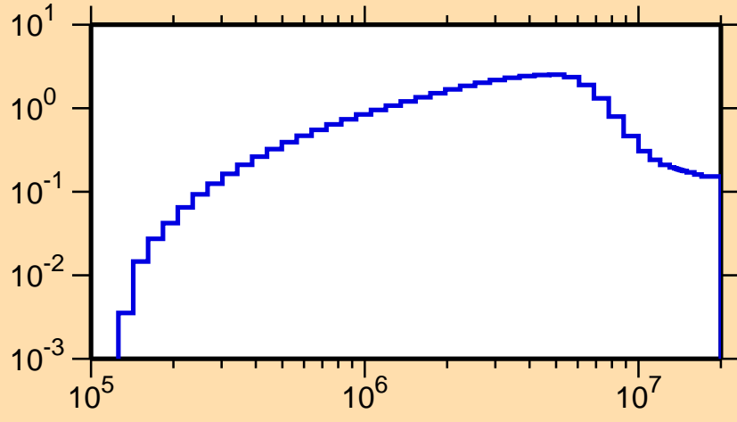
\sigma vs. E for ^{203}\text{Pt}(n,n\text{cont.})
