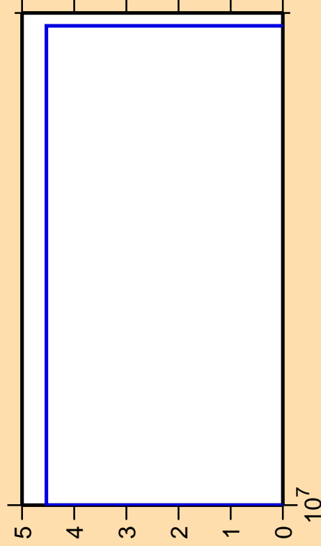
\Delta\sigma/\sigma vs. E for ^{203}\text{Pt}(n,2np)
