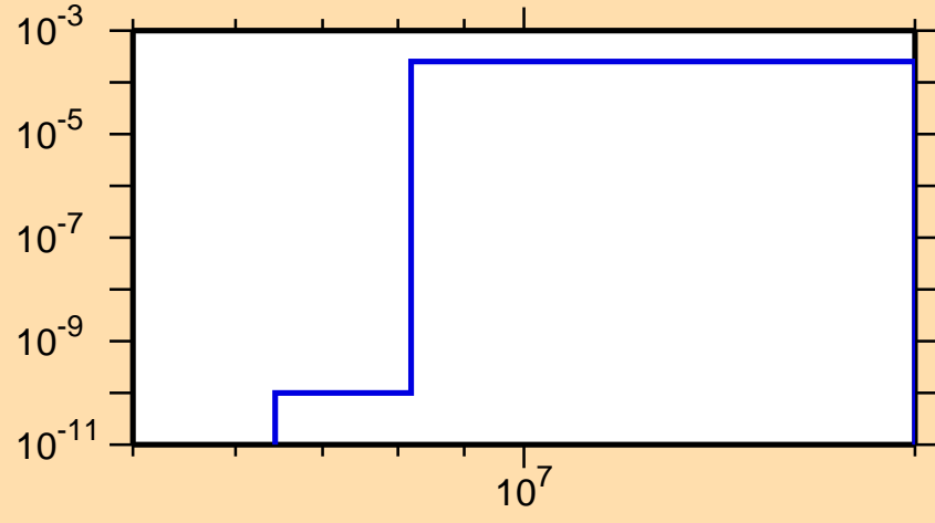
\sigma vs. E for ^{203}\text{Pt}(n,p)
