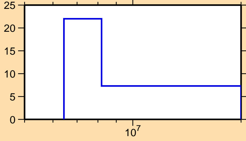
\Delta\sigma/\sigma vs. E for ^{203}\text{Pt}(n,el.)
