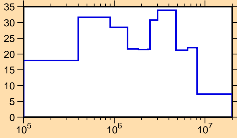
\Delta\sigma/\sigma vs. E for ^{203}\text{Pt}(n, el.)
