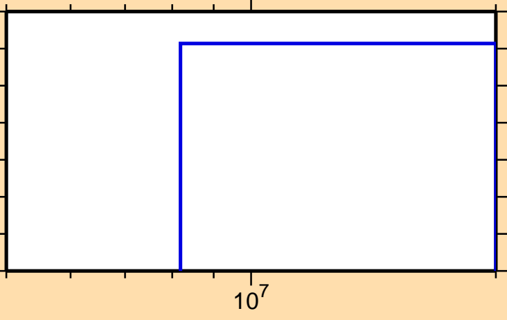
\sigma vs. E for ^{203}\text{Pt}(n,3n)
