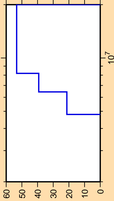
\Delta\sigma/\sigma vs. E for ^{203}\text{Pt}(n,n\text{cont.})
