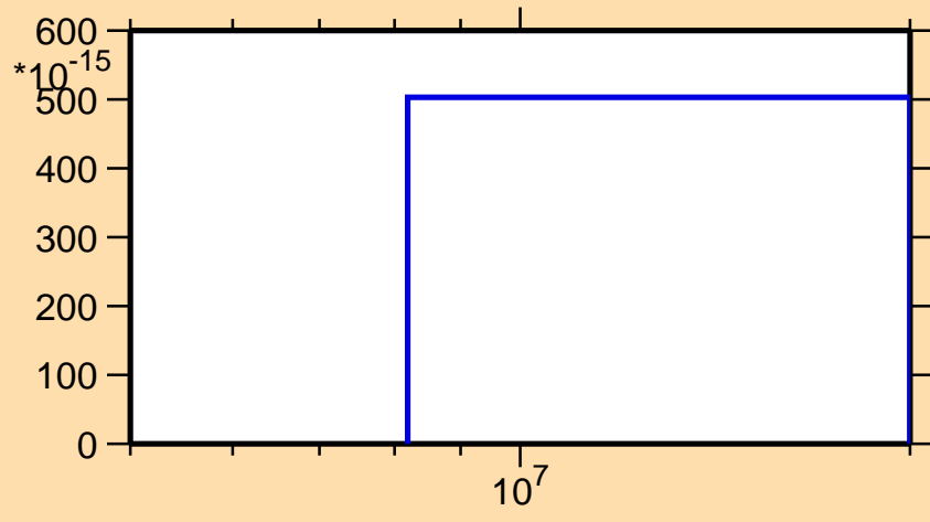
\sigma vs. E for ^{203}\text{Pt}(n,2n\alpha)
