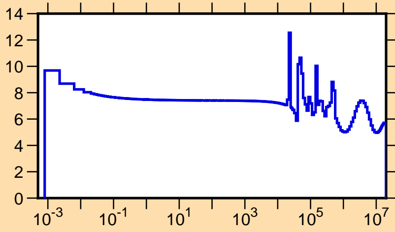
\sigma vs. E for ^{204}\text{Pt}(n,\text{tot.})
