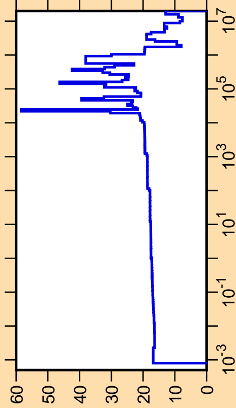
\Delta\sigma/\sigma vs. E for ^{204}\text{Pt}(n,\text{tot.})
